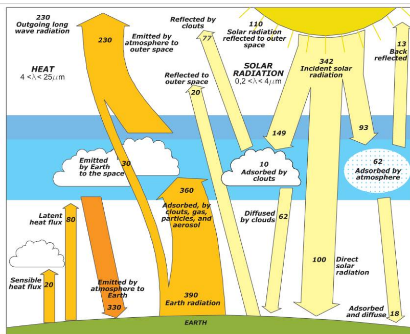
Figure 1: Earth energy flows ( \text{W/m}^2 ).
