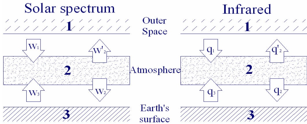
Figure 2: scheme of the irradiation heat exchange.
